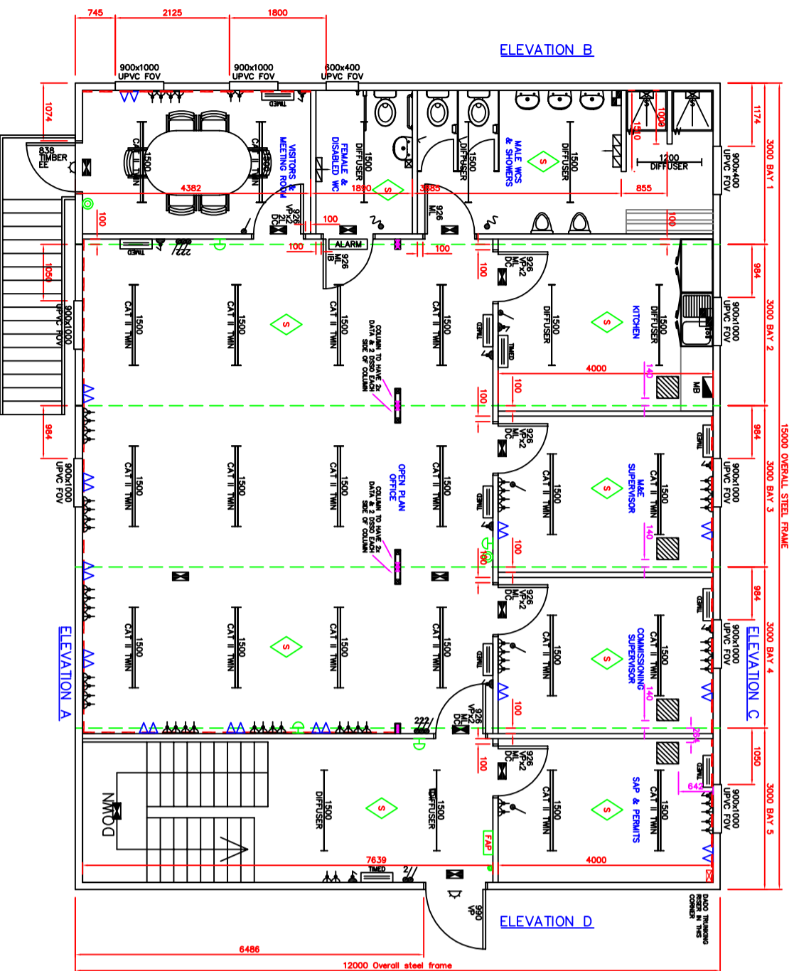
GROUND FLOOR
