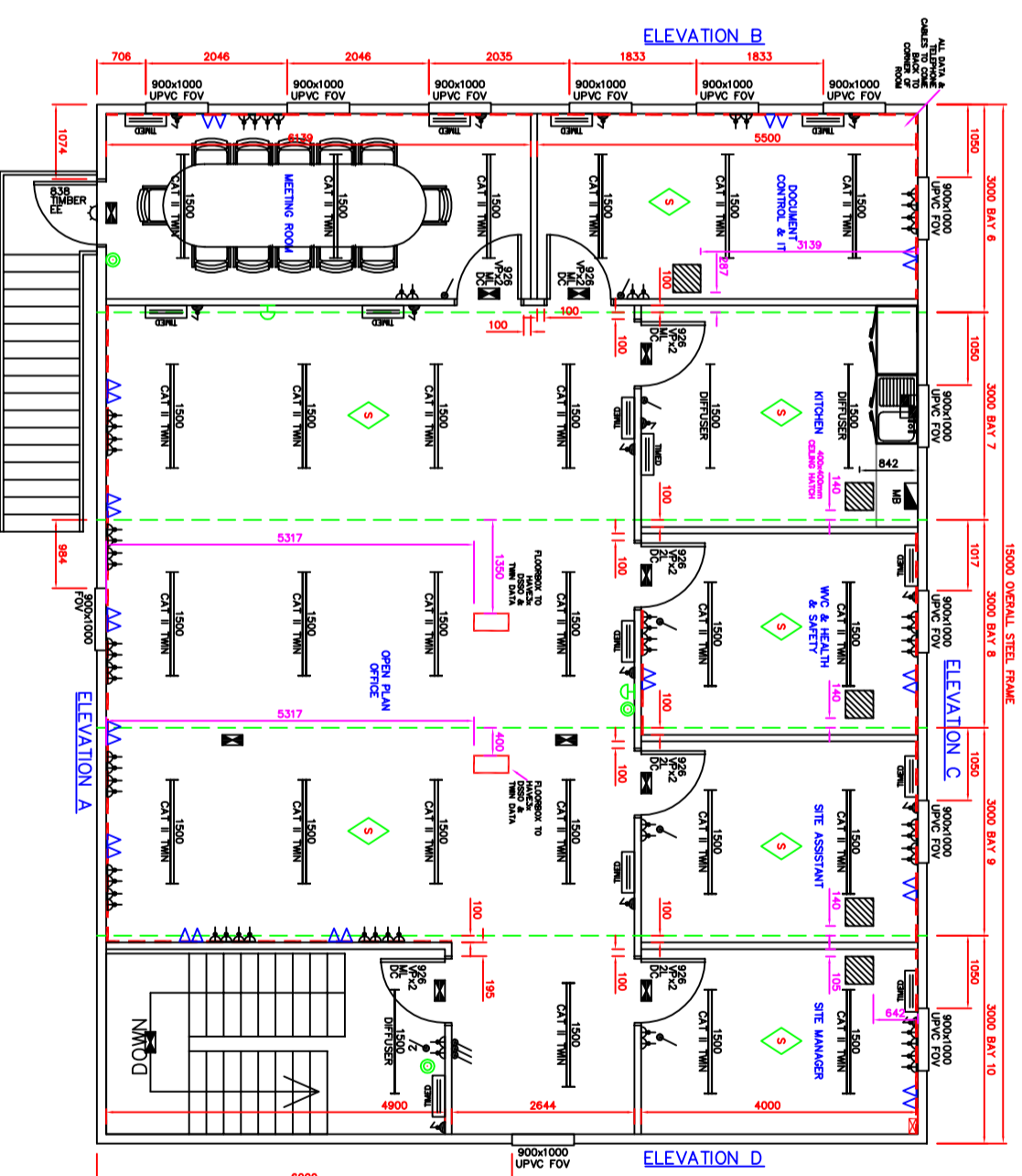
FIRST FLOOR
